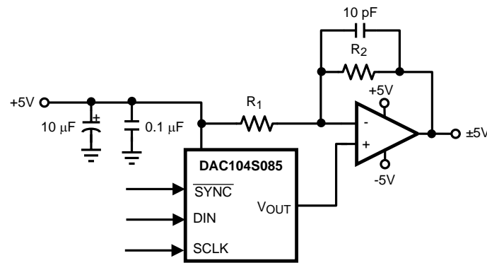
Figure 35. Bipolar Operation
